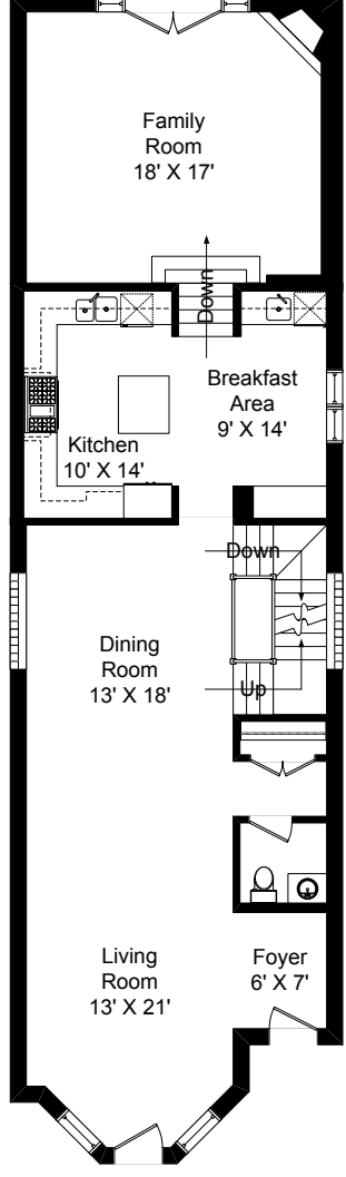
FIRST LEVEL
