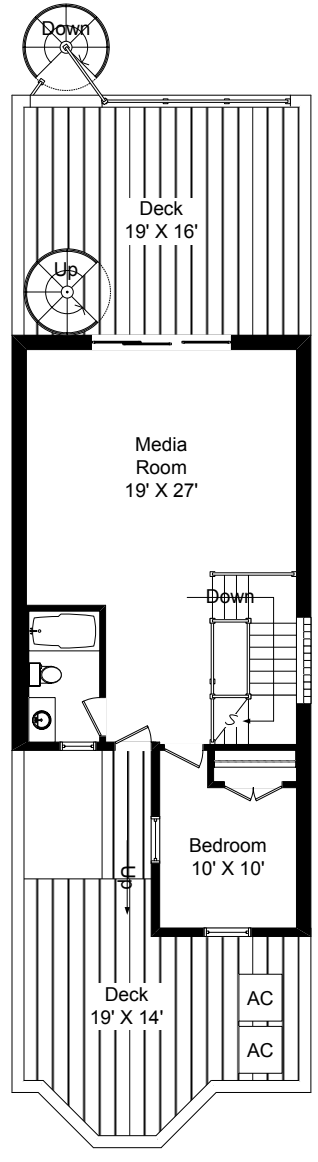
THIRD LEVEL
